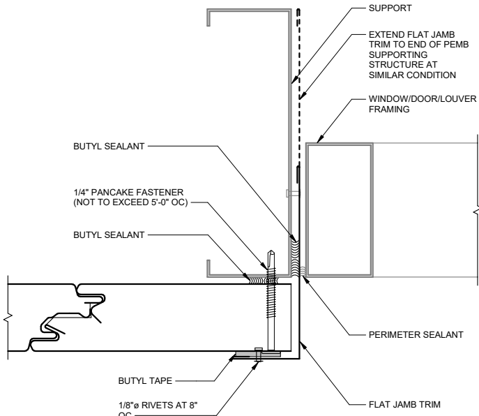
7 WALL PANEL OPENING JAMB DETAIL A-301 SCALE: 6" = 1'-0"
